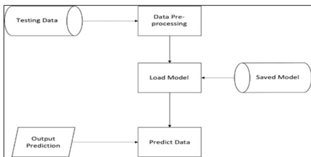
Fig. 2: Testing Phase
